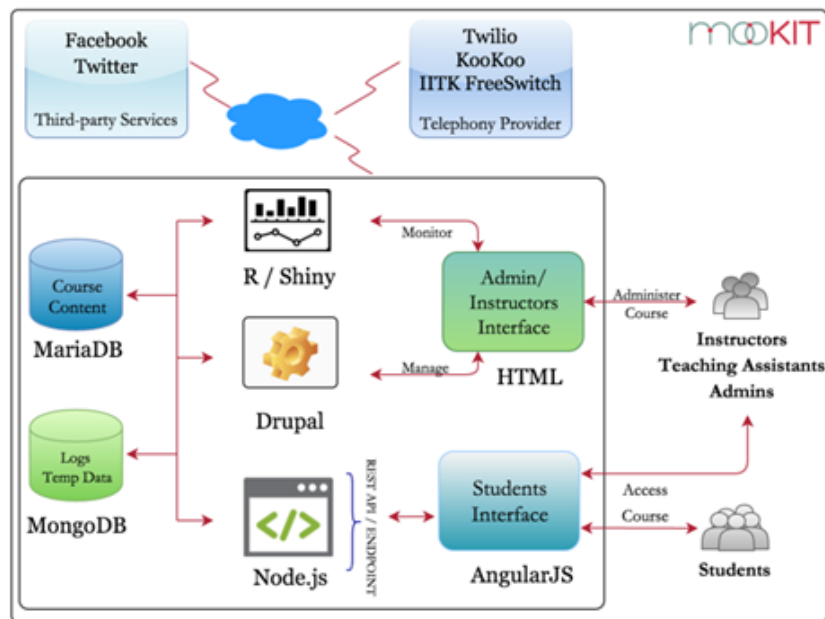
Figure 10: mookIT architecture
