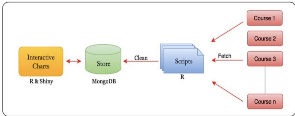
Figure 11: Analytics Processing
